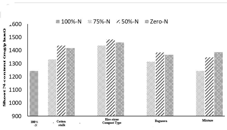
Fig. (3): Effect of organic-mineral nitrogen application on N-content of peanut shoots.
