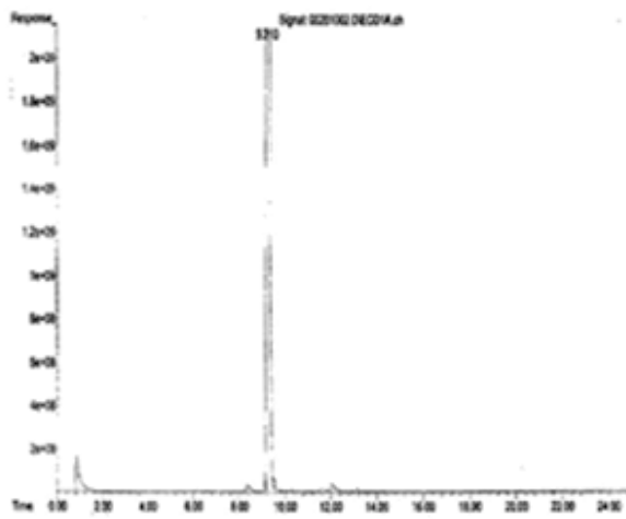
Fig (9): Standard of Amex
