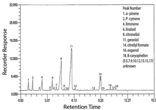
Fig (19): Chromatogram of Geranium essential oil (Roal at 750 cm 3 )
