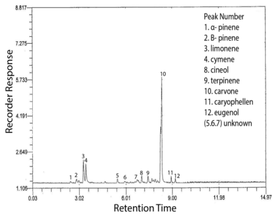
Fig 1: Chromatogram of Spearmint essential oil (control)
