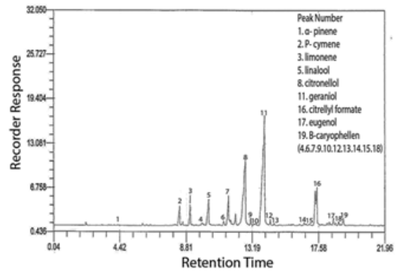
Fig (16): Chromatogram of Geranium essential oil (heoing three time)
