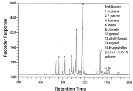
Fig (18): Chromatogram of Geranium essential oil (stomp at 1.7 l/fed)
