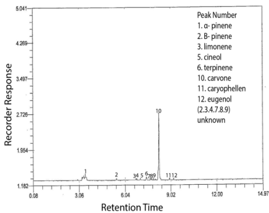
Fig 5: (Stomp at 1.7 l/fed)
