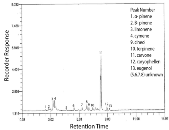
Fig 2: Chromatogram of Spearmint essential oil (Hoing three times)
